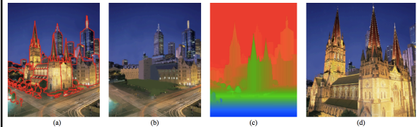
Figure 1: St Paul's Cathedral in Melbourne. (a) Image segmented into layers (boundaries in red). (b) Hidden parts manually clone brushed by the user. (c) False-color rendering of the depth of each pixel. (d) New viewpoint and relighting of the roof and towers.
