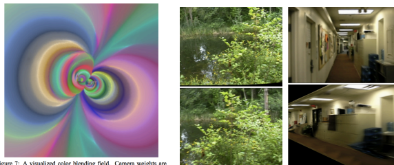
Figure 7: A visualized color blending field. Camera weights are computed at each pixel. This example is from the “hallway” dataset
