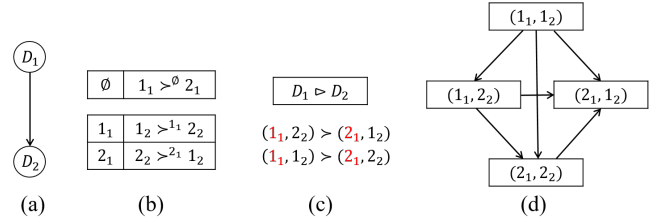
Figure 1: An O -legal lexicographic preference with an underlying CP-net, where O = [D_1 \succ D_2] .
