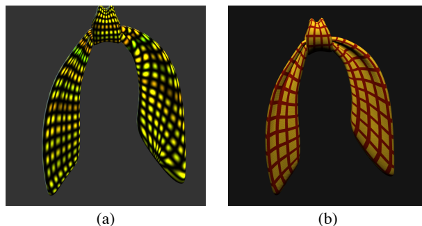
Figure 12: Gridded textures mapped onto a bandanna modeled using two subdivision surfaces. One surface is used for the knot, the other for the two flaps. In (a) texture coordinates are assigned uniformly on the right flap and nonuniformly using smoothing on the left to reduce distortion. In (b) smoothing is used on both sides and a more realistic texture is applied.
