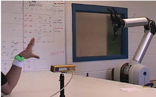
Fig. 4. Embodied interaction study: Subjects play the shadow puppet game with our 4 DOF Whole Arm Manipulator (WAM). A stereo camera is used to code the gestural language tokens of the human in real-time.
