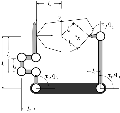
Figure 28.14: Planar hand with 2 fingers and 7 joints grasping a polygonal object.
