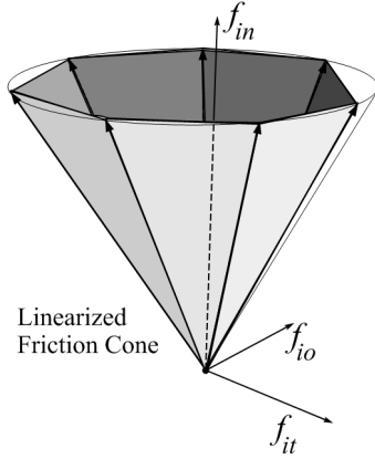
Figure 28.10: Quadratic cone approximated as a polyhedral cone with seven generators.
