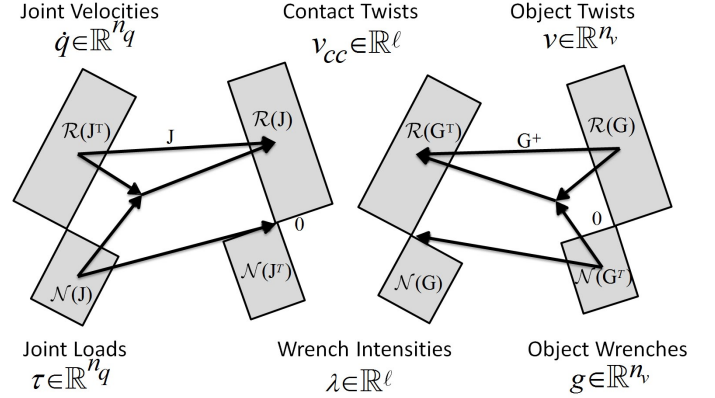
Figure 28.3: Linear maps relating twists and wrenches of a grasping system.
