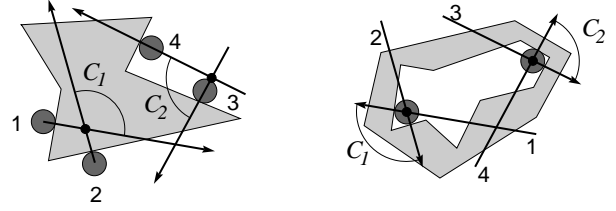
Figure 28.9: Planar grasps with first-order form closure.
