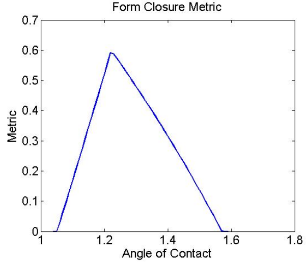
Figure 28.18: Plot of closure metric versus angle of contact 1.04 < \alpha < 1.59 .
