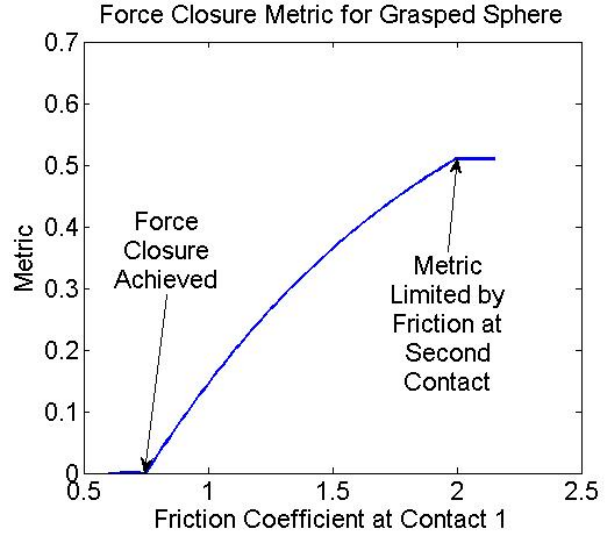
Figure 28.13: Plot of force closure metric versus friction coefficient on contact 1.
