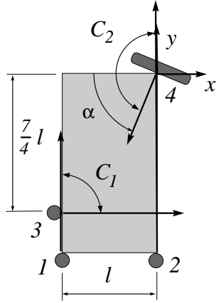
Figure 28.17: Planar grasp with first-order form closure if 1.052 < \alpha < \frac{\pi}{2} .
