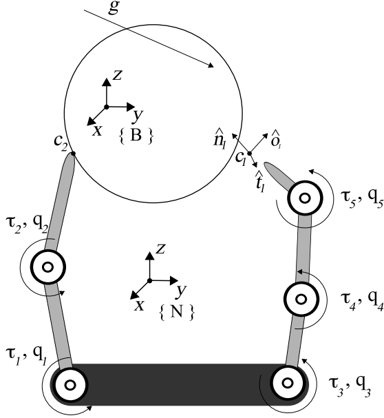
Figure 28.2: Main quantities for grasp analysis.
