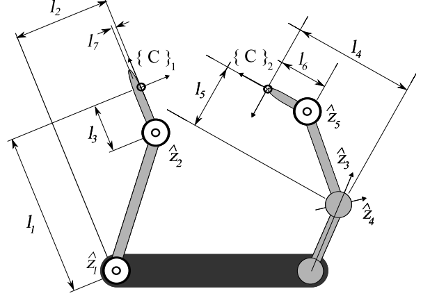
Figure 28.12: Relevant data for the Hand Jacobian
