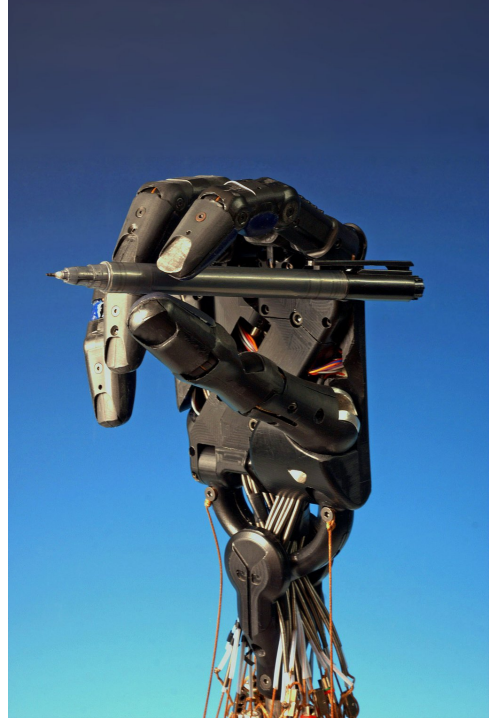
Figure 28.6: This grasp has a force closure grasp appropriate for dexterous manipulation.
