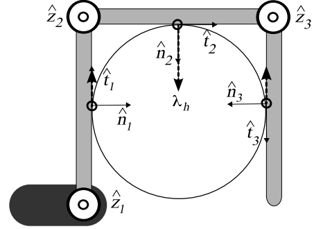
Figure 28.15: A sphere grasped by a finger with three revolute joints. The force direction \lambda_h (dashed line) is a force that belongs to both \mathcal{N}(\mathbf{G}) and \mathcal{N}(\mathbf{J}^T) and causes hyperstaticity.
