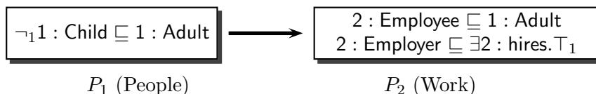
Figure 1. Semantic Importing
