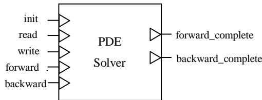
Figure 5: A Process-port View of the Continuous Simulation
