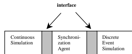
Figure 2: Linking Two Simulations
