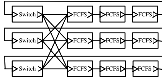
Figure 3. A CQN with 3 Switches and 9 FCFS Servers.
