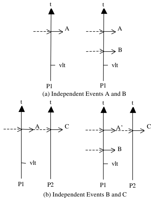
Figure 2. Supercriticality and Independent Events
