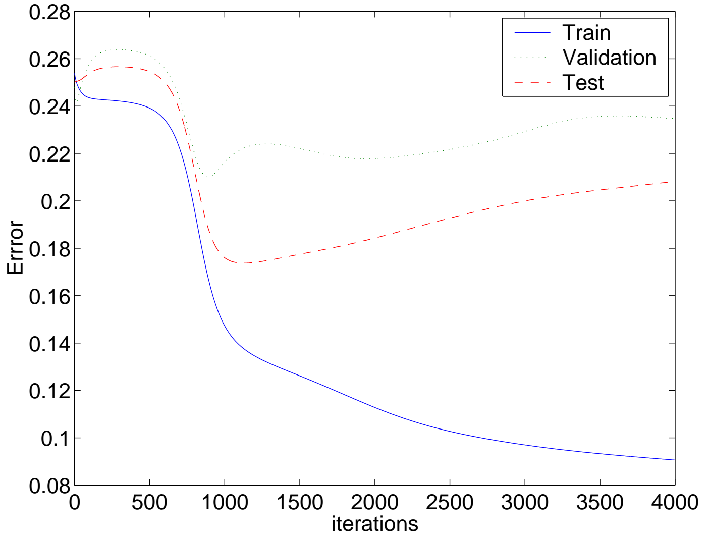
Training, Test And Validation with Nh=10, 35/5 Train/Val Split
