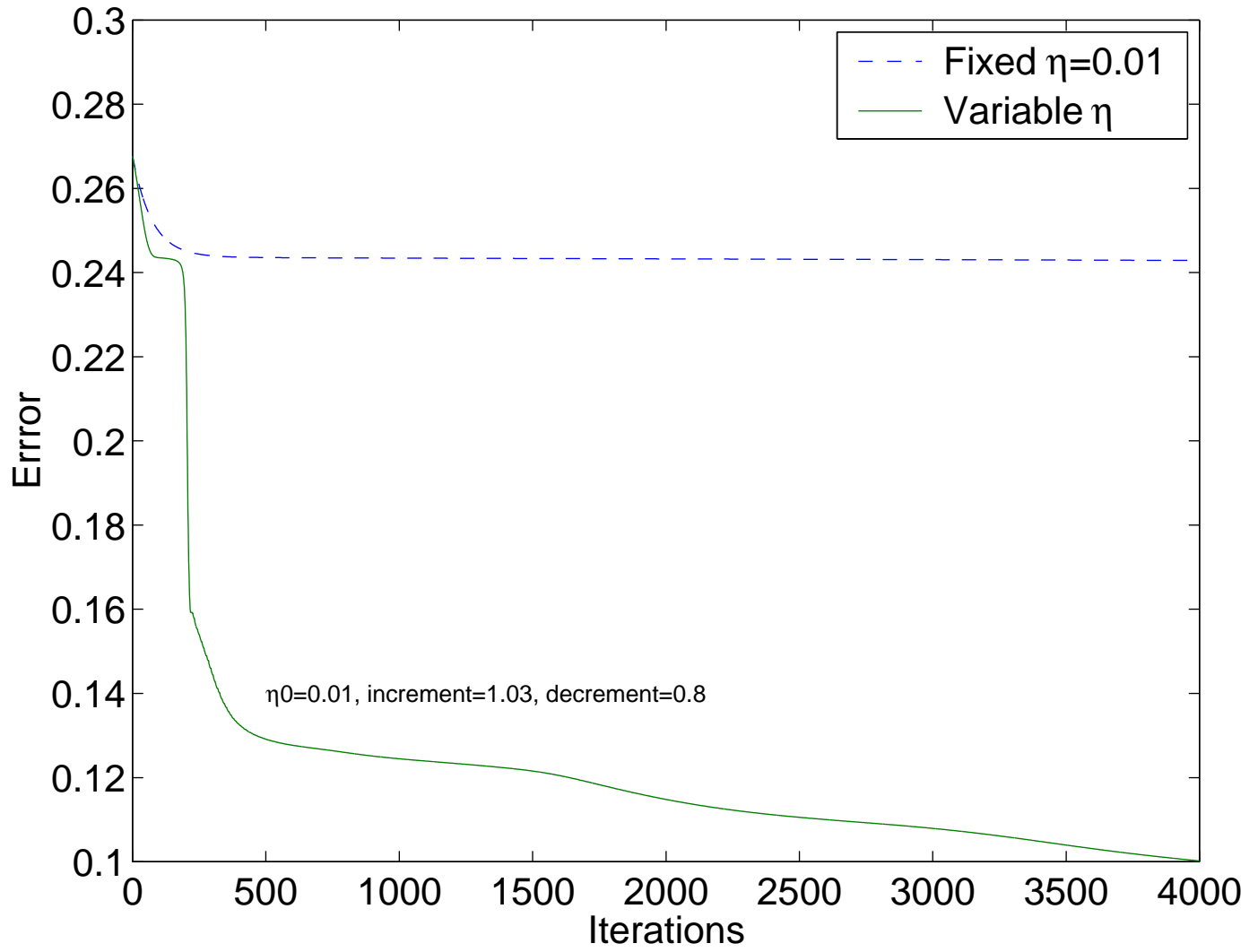
Training Errors for Fixed and Variable Learning Rate
