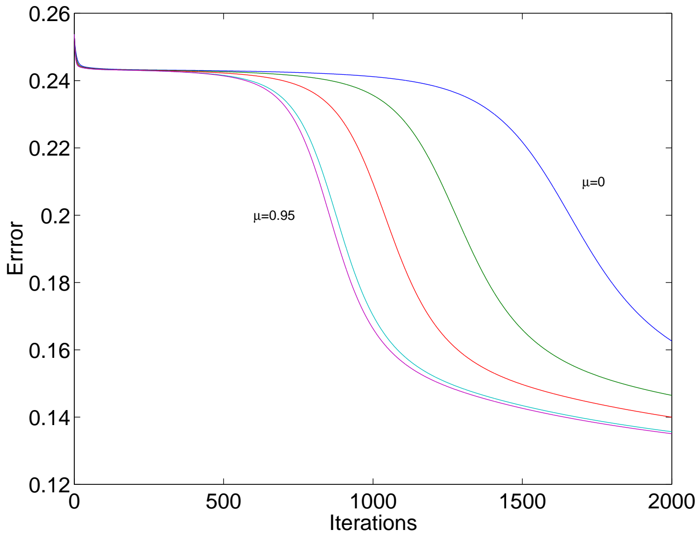
Training Error Dependence on Momentum Parameter, \eta=0.1
