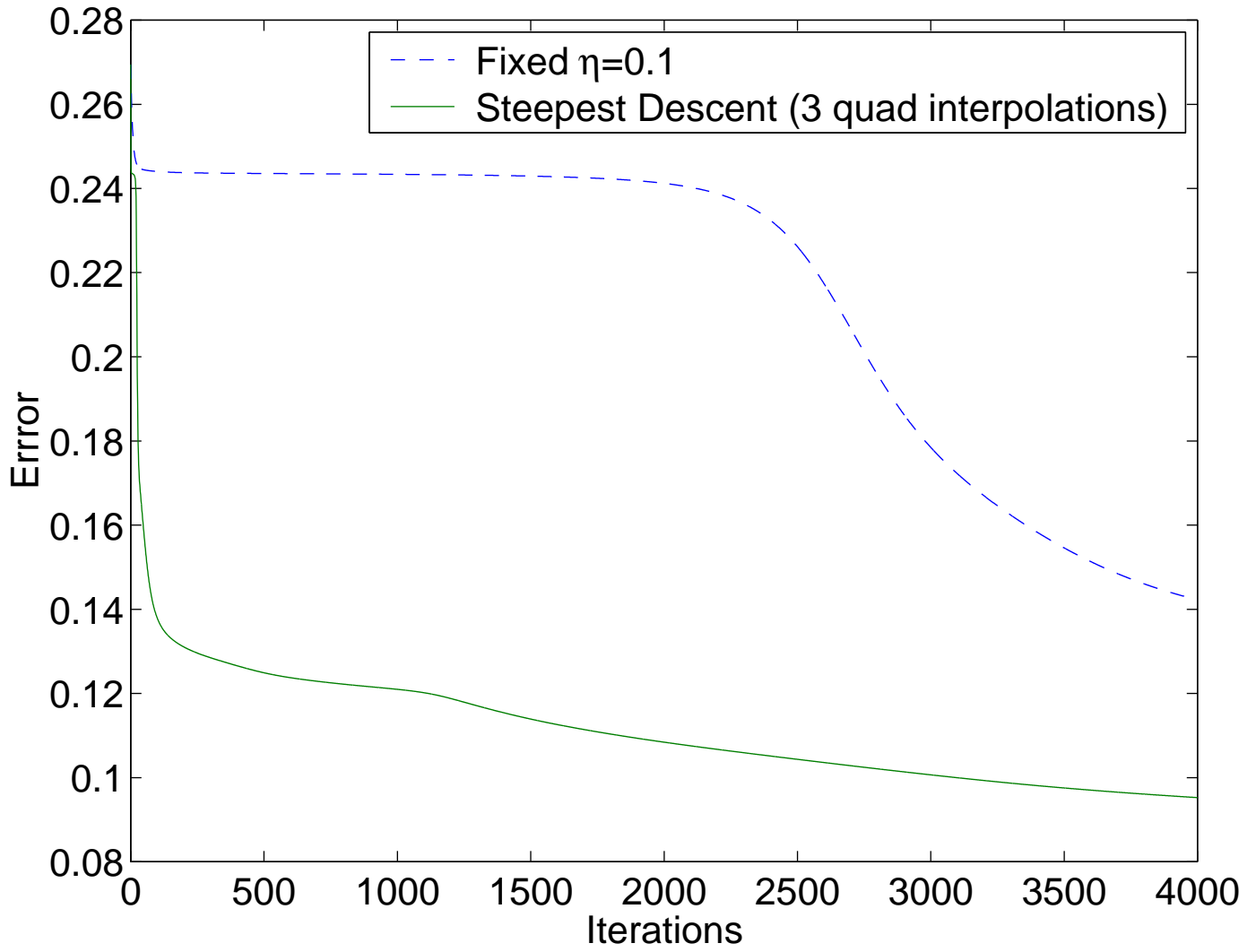
Training Error For Gradient Descent and Steepest Descent
