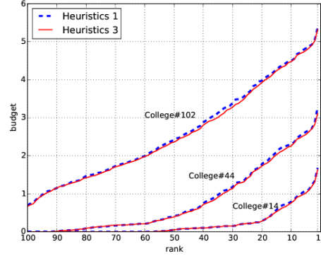
Figure 5: Heuristics 1 & 3 for 15D USNews data.
