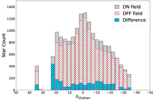
Figure 3. Histogram of the turnoff star counts as a function of angle along the Orphan stream. The data in this figure is the same as in Figure 5 of Newberg et al. (2010). The black histogram shows the star counts on the Orphan Stream, the red the star counts in a region of the sky around the Orphan Stream, and the filled histogram shows the difference. The difference histogram is used in our optimization as the number of stars as a function of angle along the stream.
