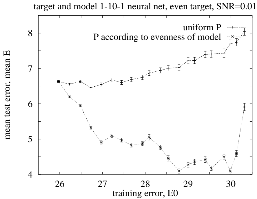
Figure 5: The mean test error versus training error of a nonlinear model for a given even target and training set. The mean test error increases as the training error increases when all models with the same training error are given equal probability of selection. Choosing the models with the smaller evenness error with higher probability reduces the mean test error.
