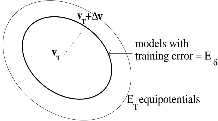
Figure 1: The models with training error E_\delta = E_T(\mathbf{v}_T) + \delta form the early stopping set at training error level E_\delta .
