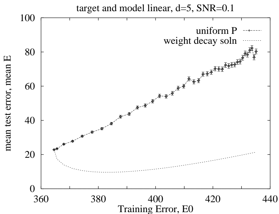
Figure 4: The mean generalization/test error versus training error of a linear model for a given target and training set. The mean generalization error increases as the training error increases when all models with the same training error are given equal probability of selection. When the weight decay parameter is small enough, choosing the weight decay solution with probability 1 and all other models with the same training error with probability 0 improves the generalization error.
