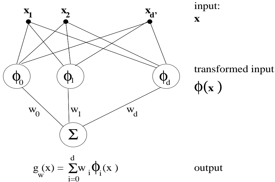
Figure 2: General linear model.
