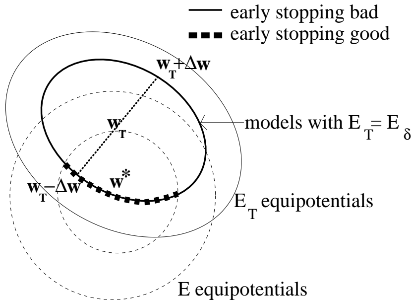
Figure 3: Early stopping at a training error \delta above E_T(\mathbf{w}_T) results in higher generalization error when all models having the same training error are equally likely to be chosen as the early stopping solution.
