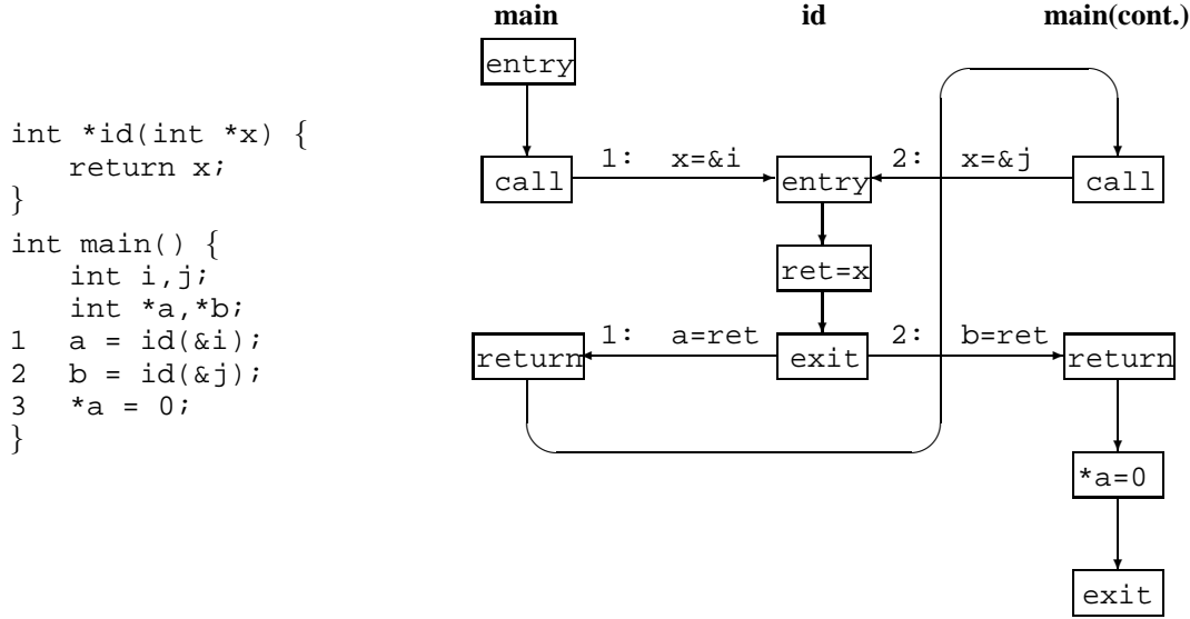
Figure 5. Sample program and its interprocedural control flow graph.
