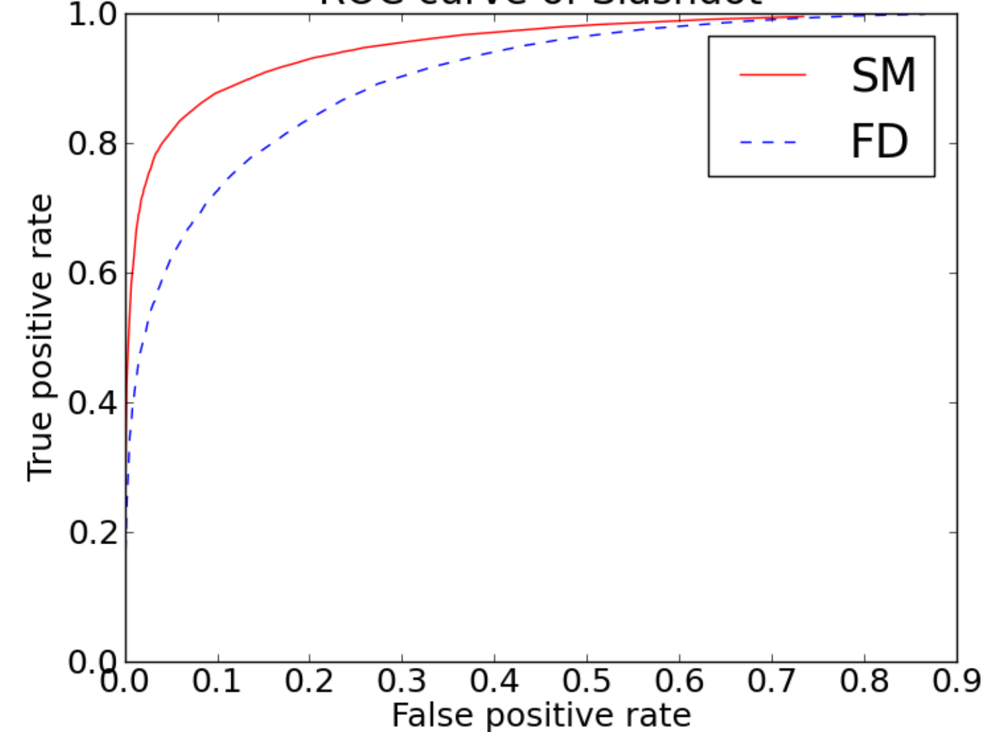
ROC curve of Slashdot
