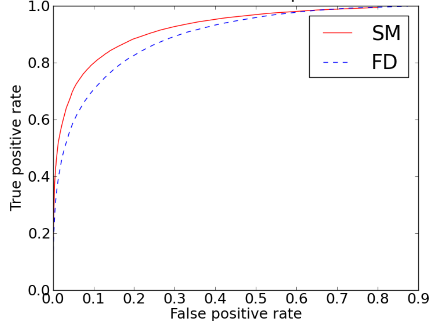
ROC curve of Wikipedia
