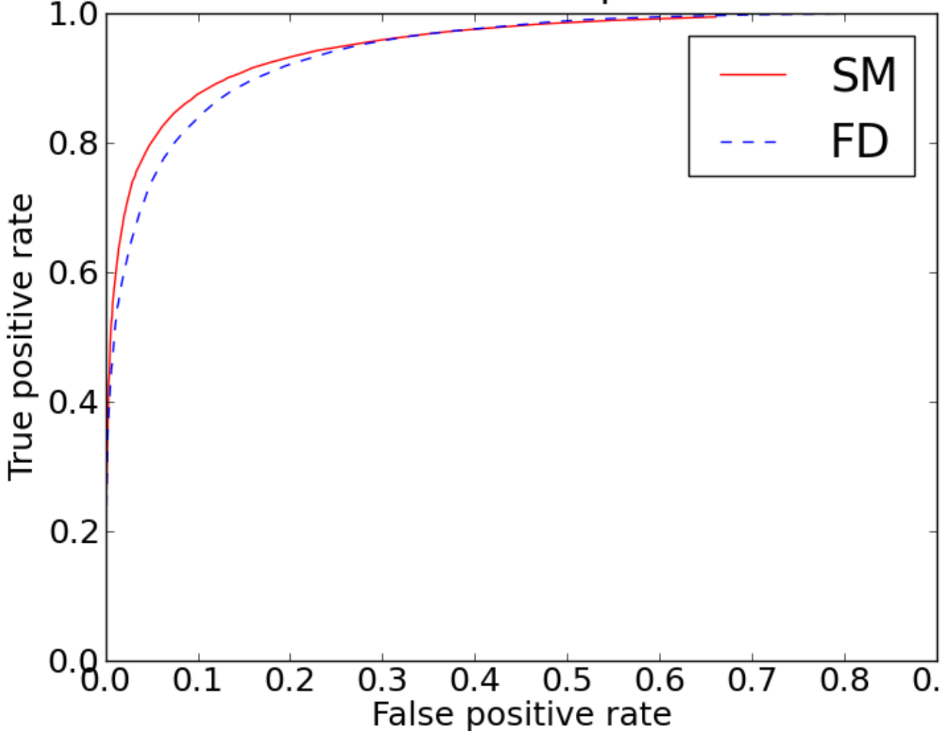
ROC curve of Epinions
