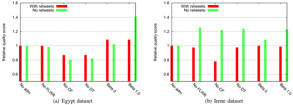
Fig. 3. Relative quality scores across different admission control schemes.
