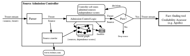
Fig. 1. Schematic model of the admission controller with Apollo’s pipeline.
