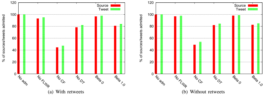
Fig. 4. Admission controller statistics for different admission schemes (Egypt dataset).
