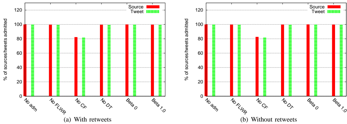
Fig. 5. Admission controller statistics for different admission schemes (Irene dataset).
