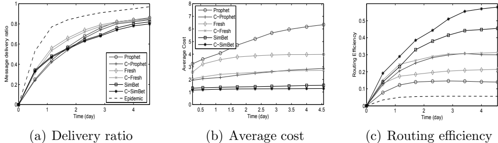
Figure 7: Comparison using Cambridge traces
