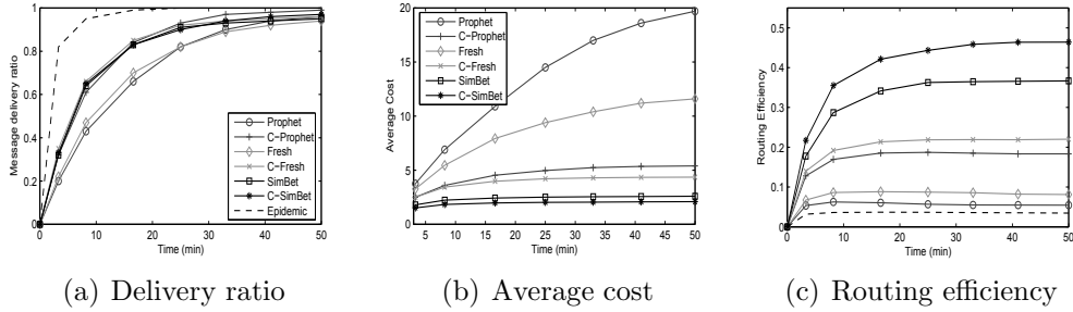
Figure 6: Comparison using RollerNet traces
