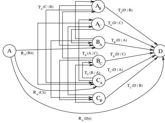
Figure 4: A sample DTN graph with 4 nodes where A is the source and D is the destination.
