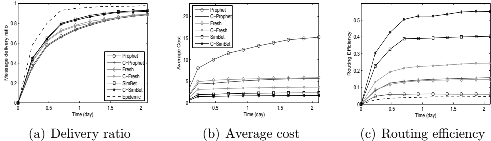
Figure 8: Comparison using Haggie traces
