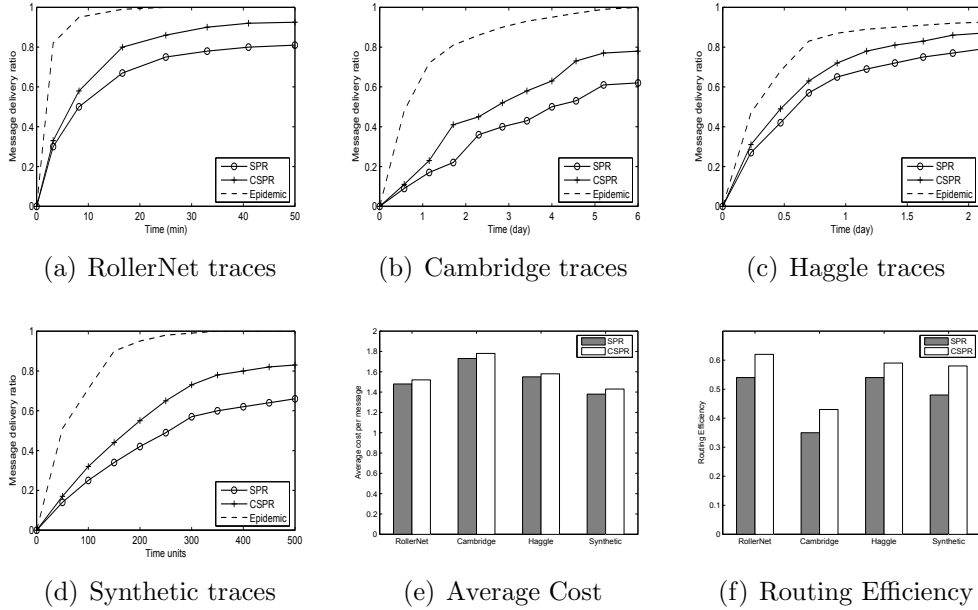
Figure 5: Comparison of SPR and CSPR: Message delivery ratio (a-d), Cost (e) and Routing Efficiency (f).
