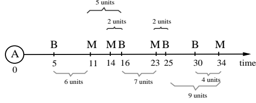
Figure 2: Example meeting times of node A with nodes B and M . Upper and lower values are used to compute \tau_A(B|M) and \tau_A(M|B) , respectively.
