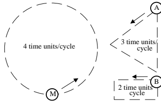
Figure 1: An example cyclic MobiSpace with a common motion cycle of 12 time units.
