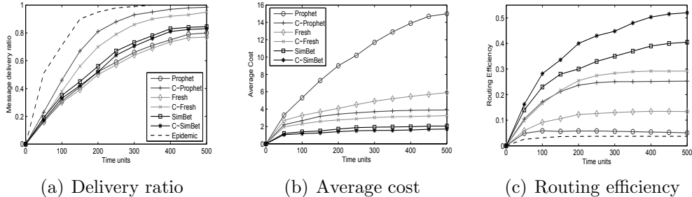
Figure 9: Comparison using Synthetic traces
