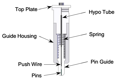
Figure 8. Model of Pin Insertion Tool
