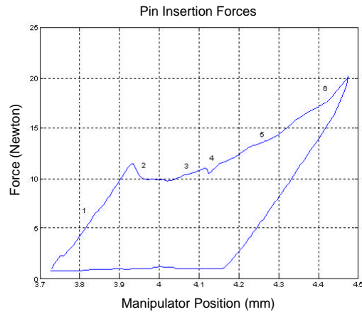
Figure 14. Pin Insertion Forces
