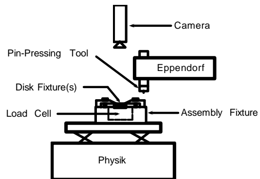
Figure 2. Schematic of Pin-Pressing Cell
