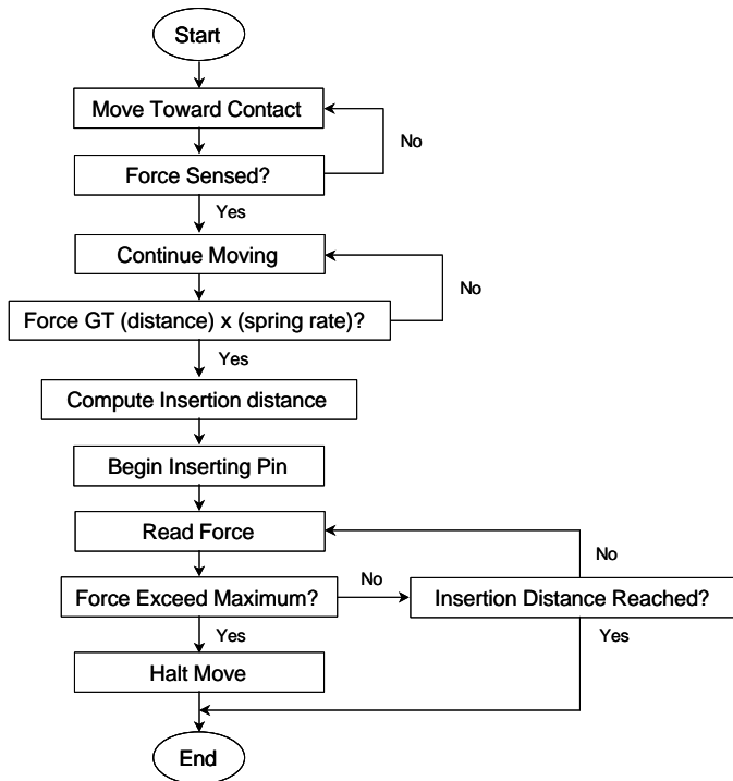
Figure 15. Position/Force Control Algorithm
