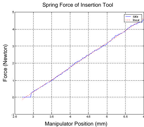
Figure 13. Spring Force of Insertion Tool
