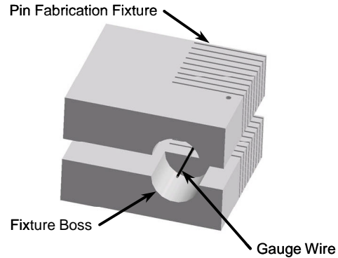
Figure 4. Model of Fixture
