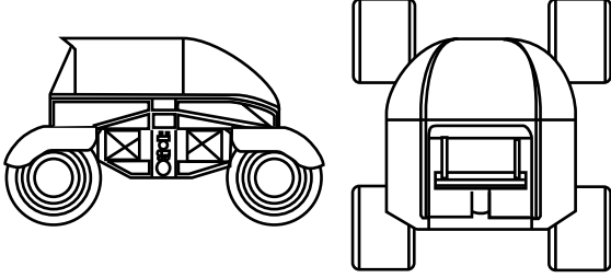
Figure 10: Profile of the Nomad rover.
