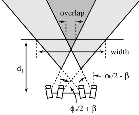
Figure 4: Width of coverage. Two pairs of cameras provide a greater area of stereo coverage. We must have a certain width of stereo coverage at the lookahead distance; consequently, the stereo coverage must also overlap at the lookahead distance.
