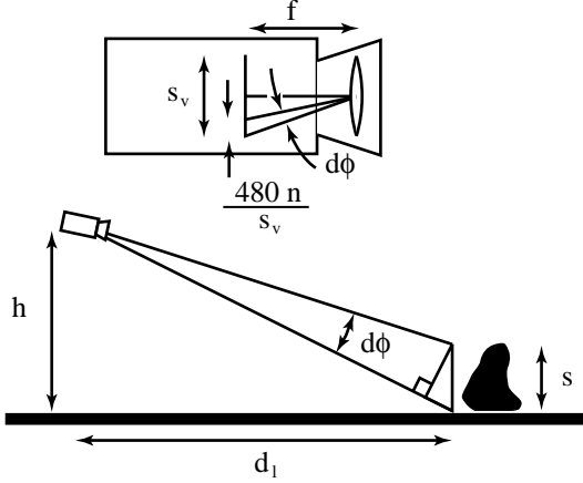
Figure 7: Resolution. The number of pixels on an object of height s at the look-ahead distance can be determined by comparing similar triangles formed by the camera and the object's image and by the camera and the object.
