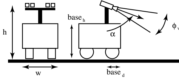
Figure 1: Configuration of the stereo mast. We assume that the location of the mast, i.e. the distance from the front of the robot ( base_d ) and the height of its base ( base_h ), is given. Our optimization will determine the height of the camera mast (actually the height of the cameras above the ground, h ), the elevation of the cameras ( \alpha ), and the focal length of the lens ( f ). The focal length will determine the vertical field of view ( \phi_v ).
