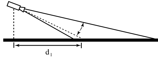
Figure 9: Stereo coverage approximation. An approximate measure of stereo coverage is the product of the width of coverage at the look-ahead distance and the angle of coverage beyond the look-ahead distance.
