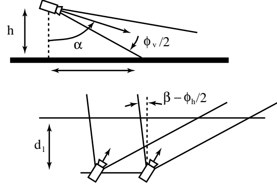
Figure 6: Lookahead. In order to see the ground at the lookahead distance, the cameras must point downwards far enough. However, the further the cameras are rotated outwards, the lower the elevation of the cameras must be.
