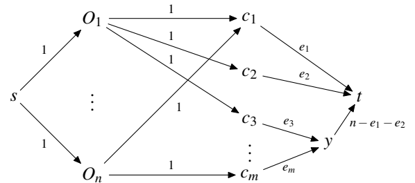
Figure 1: F_{\{c_1, c_2\}}^{\vec{e}} .
