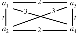
Figure 1: A similarly function d_t where t > 0 .
