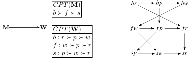
(a) A CP-net \mathcal{N} .
