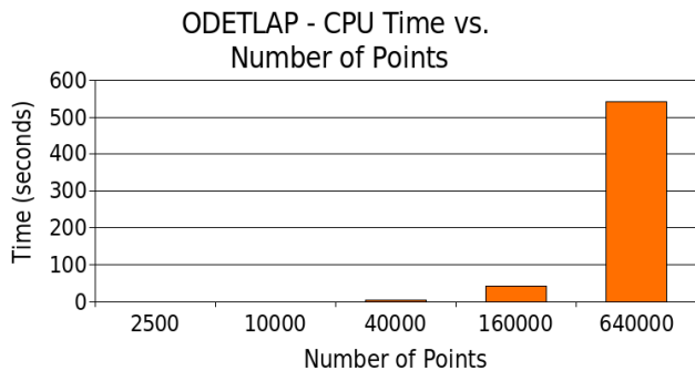
Figure 5: ODETLAP performance on a single large patch on grid with 1% known (original) points. The “Number of Points” refers to the number of points in the reconstructed grid. The calculation time grows quadratically with the number of points, and it takes nearly 10 minutes to process an 800 \times 800 grid.
