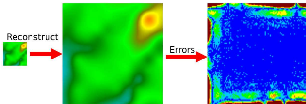
Figure 8: Due to incomplete data, ODETLAP results in errors near the borders of a patch when we compare the results from the non-patch ODETLAP method with the results from running ODETLAP on a small patch. The error plot on the right shows correct results in blue, and elevation differences of 5 or more units (meters) in red.
