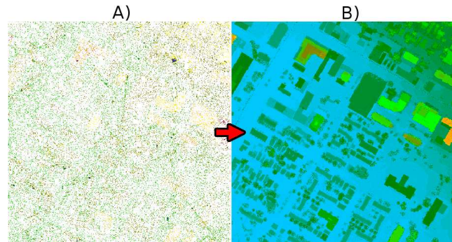
Figure 1: Our parallel version of ODETLAP was used to generate a dense 10000 \times 10000 raster (B) from raw urban LIDAR data consisting of 13 million points (A) quickly on a cluster of 128 2.6 GHz AMD Opteron processors.
