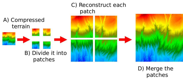
Figure 7: In the patch ODETLAP method, we take the compressed terrain (A), and divide it into patches (B). Next, we run ODETLAP on each patch individually, which reconstructs a small portion of the entire elevation map (C). Finally, we merge all of the patches into the final approximated solution (D).
