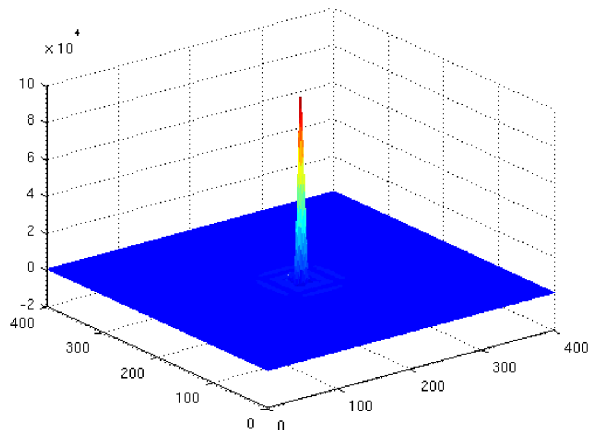
Figure 6: Altering a single known point in the terrain has a limited radius of impact during reconstruction. This plot shows the per-pixel difference between the ODETLAP solution (using a 1% subsampling of a 400 \times 400 elevation map with elevations ranging from 219 to 1040) and the ODETLAP solution for the same data with the central point edited by setting its elevation to 100,000. The difference in the solutions was restricted to a 62 \times 62 area around the altered point, with 88% of the affected points concentrated in the center 30 \times 30 area.
