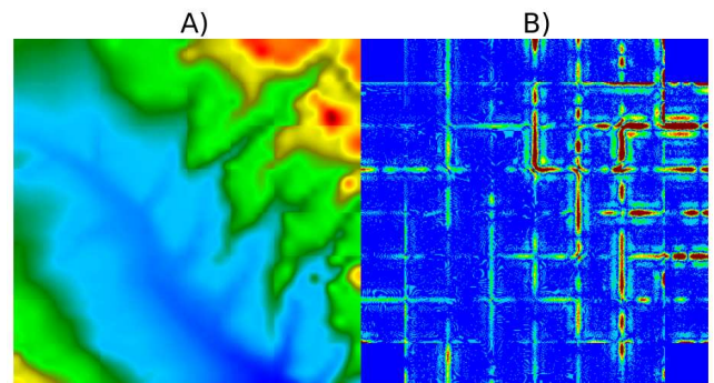
Figure 10: A simple averaging of overlapping patches reduces some of the border error of the reconstructed terrain. A) shows the image that has been merged by averaging, and B) shows the errors. Notice the visible discontinuities where patch edges are averaged.
