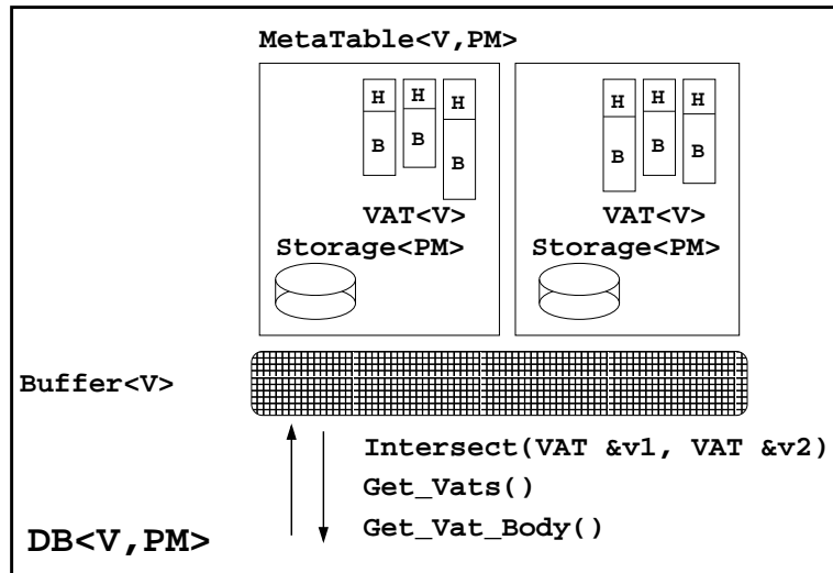
Fig. 3. DMTL: High level overview of the different classes used for Persistence
