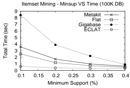
(a) Itemsets: Varying Minsup
