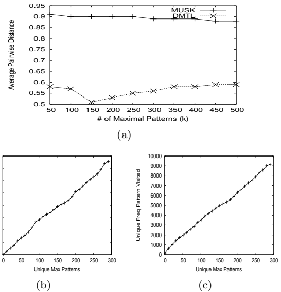
Figure 9: MUSK Quality & Time
