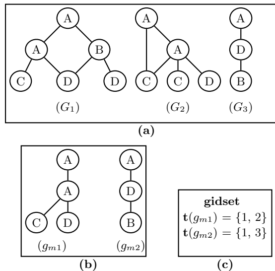
Figure 1: (a) Graph database with 3 graphs (b) Maximal frequent graphs (a) with support 2 (c) gidset of the maximal graphs g_{m1} and g_{m2}
