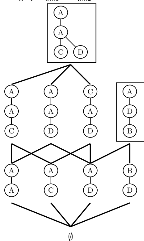
Figure 2: Partial Order Graph of Frequent Subgraphs
