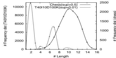
(b) Length Distribution of Maximal patterns
