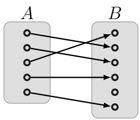
1-to-1; not onto (injection, A \xrightarrow{INJ} B ) |A| \leq |B|
