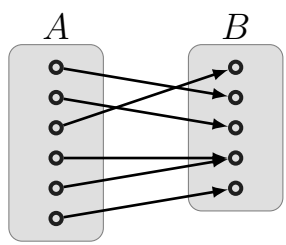
onto; not 1-to-1 (surjection, A \xrightarrow{SUR} B ) |A| \geq |B|
