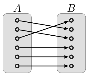
1-to-1 and onto (bijection, A \xrightarrow{BIJ} B ) |A| = |B|
