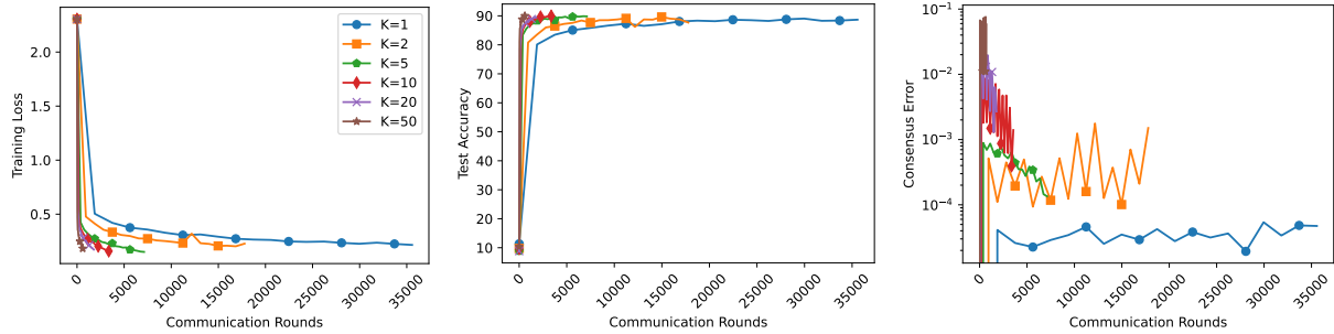
(b) FashionMNIST reduction in communication rounds.
