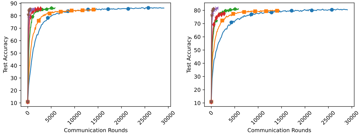
(b) AdaGrad (left) and AMSGrad (right) on CIFAR-10 with Top- k compression of 40%.
